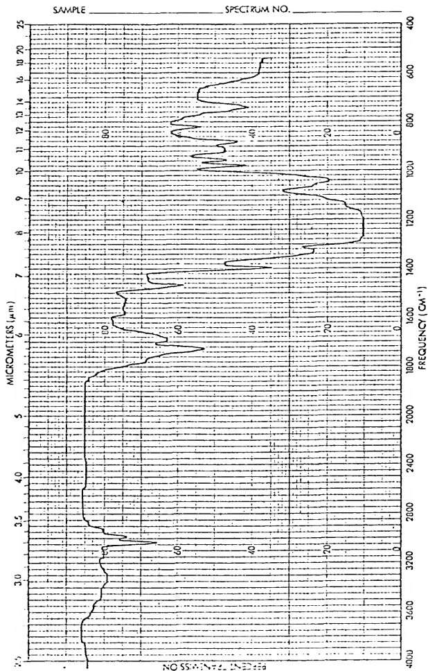
Figure 50 - Infrared Spectrum of Polymer from Reaction of \text{CF}_3\text{NO} and \text{CF}_2=\text{CFCH}=\text{CHCH}_3
